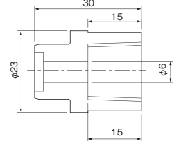
●メスねじ受口 (Rc 1/4・3/8) Female Thread (Rc 1/4・3/8)
